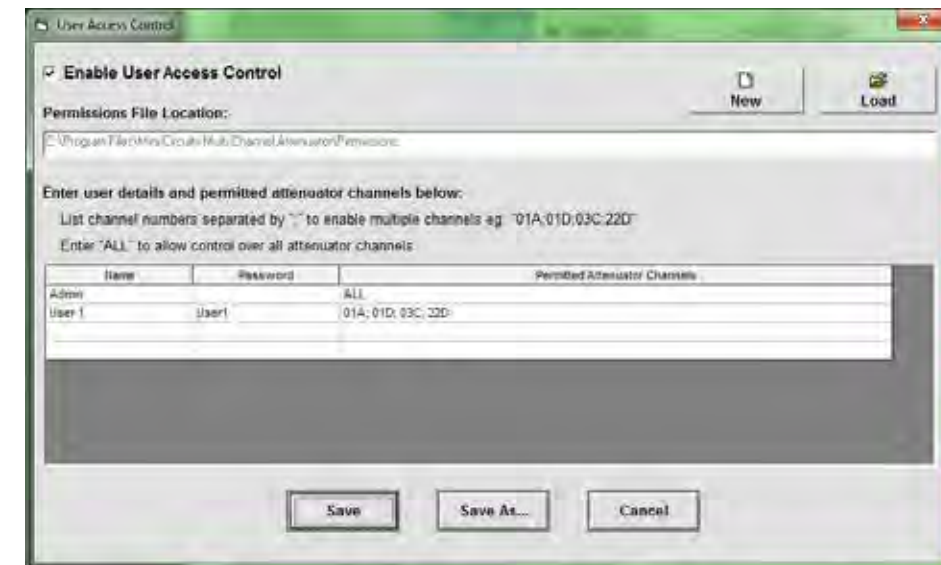
User access control menu
