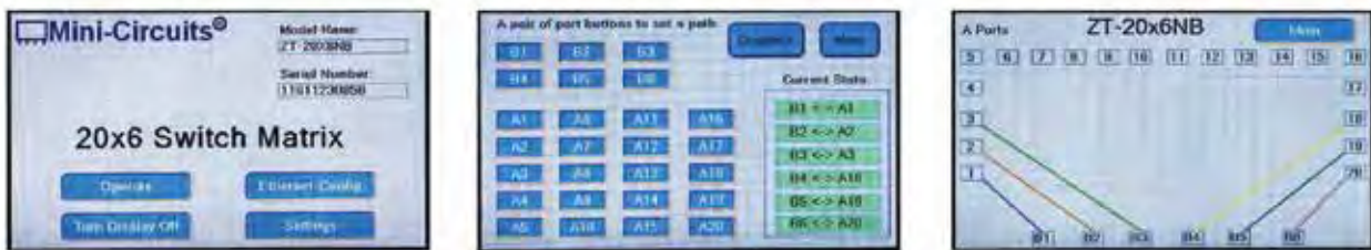
ZT-20X6NB GUI touch screen displays
