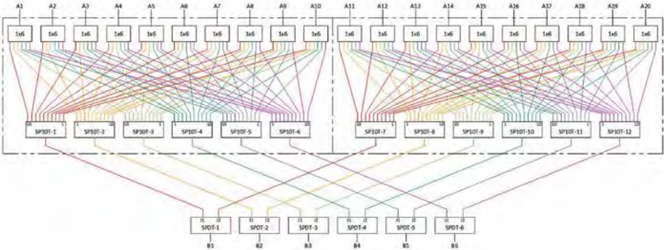
Functional Schematic
