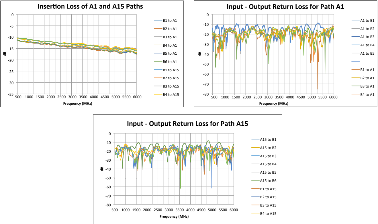
ZT-20X6NB Curves
