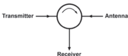
FIGURE 2 - Duplexor
